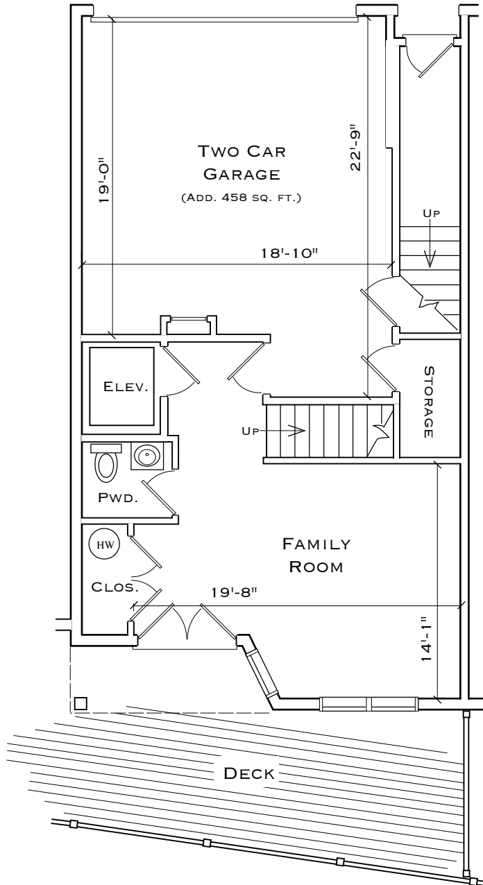
MAIN LEVEL 476 SQ. FT.
